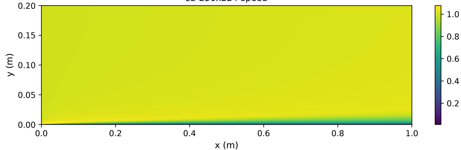
sa-256x224 speed
