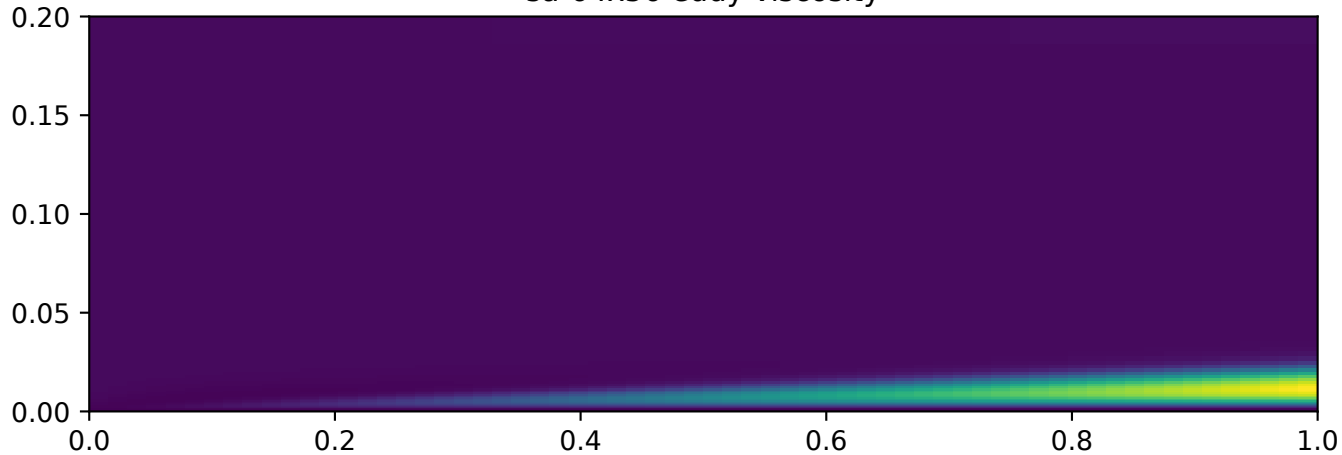
sa-64x56 eddy-viscosity
