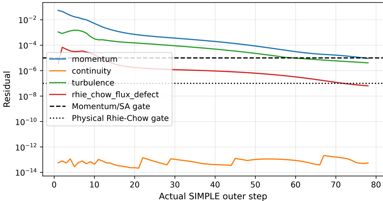
sa-64x56 cpu convergence
