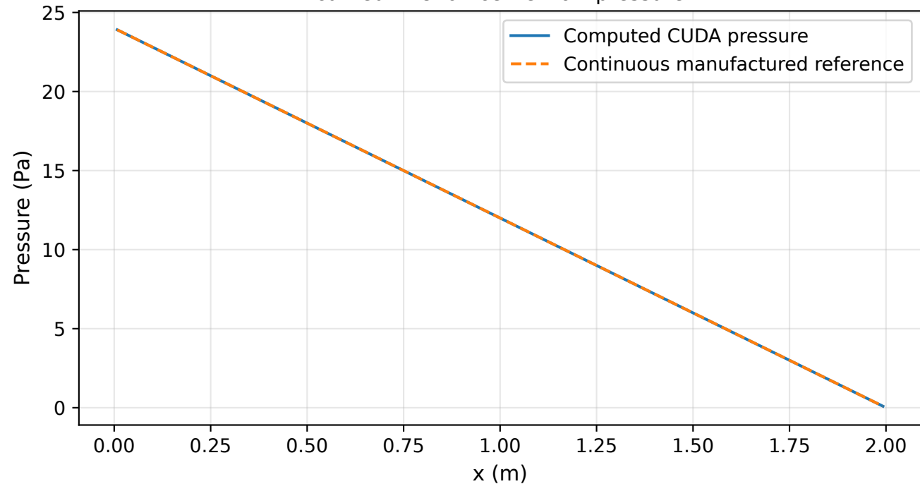
curved-128x64 center-row pressure
