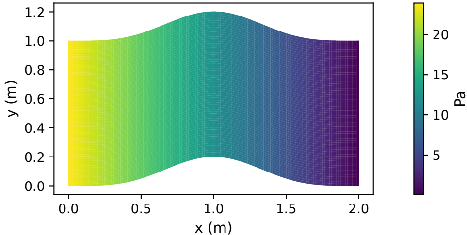
curved-128x64 pressure
