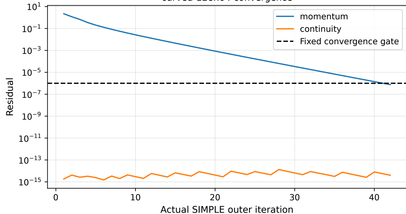
curved-128x64 convergence
