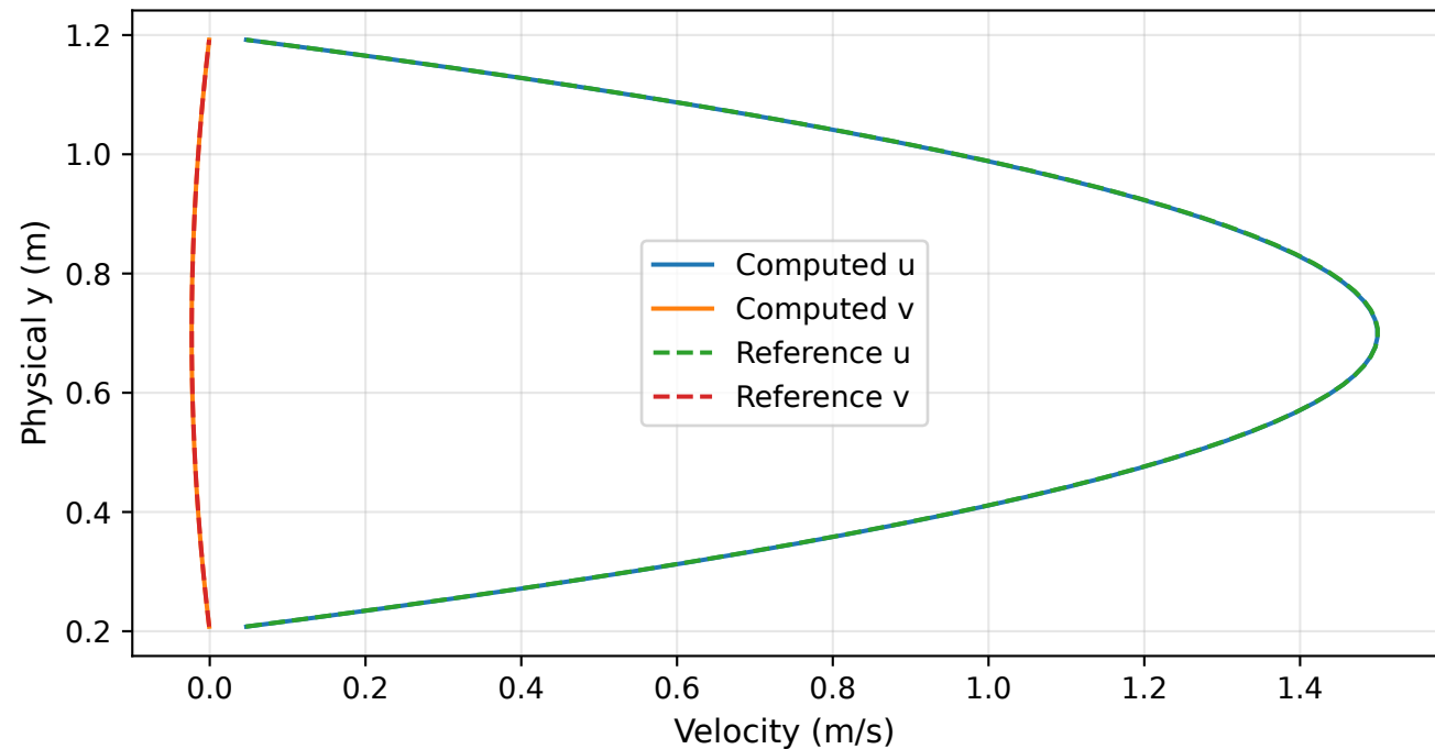
curved-128x64 mid-channel profile
