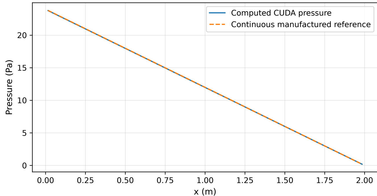
curved-64x32 center-row pressure
