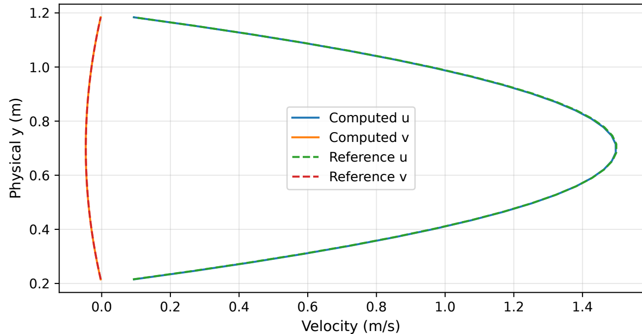
curved-64x32 mid-channel profile
