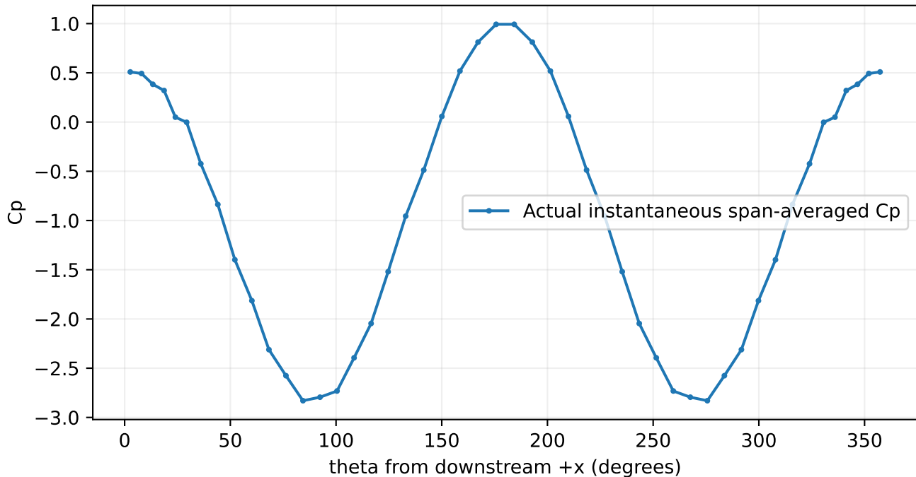
Startup surface C_p ; reference raw points not ingested
