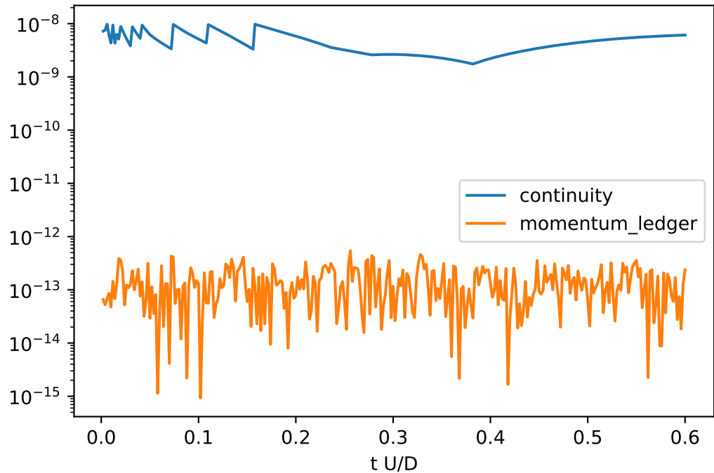
Independent mass and momentum ledgers
