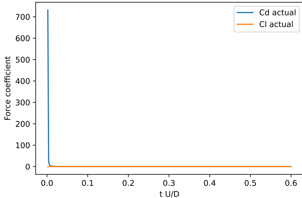
Startup force, not time-averaged reference
