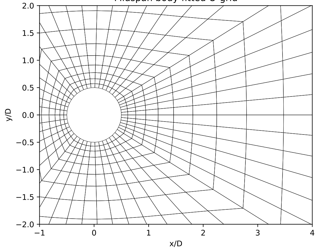
Midspan body-fitted O-grid
