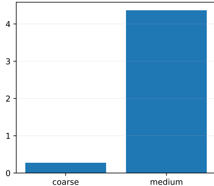
Mesh/operator/LU setup seconds
