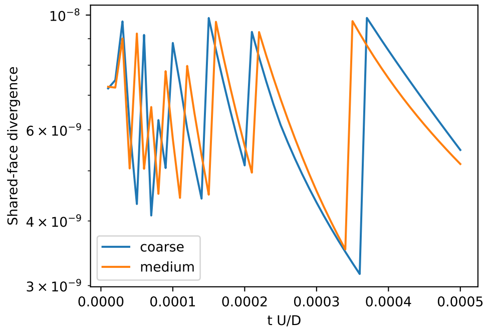
Matched 50-step startup at dt=1e-5 : NOT converged
