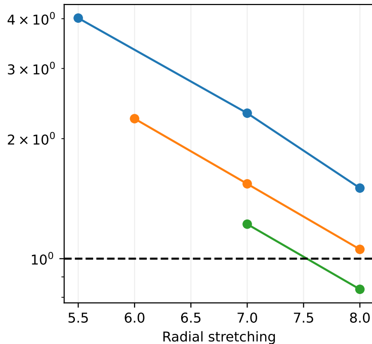
Initial y+ indicator; NOT qualification
