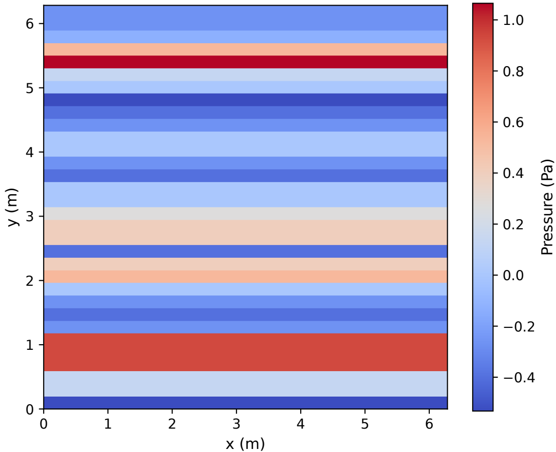
advected-shear-lbm 32x32: first z cell slice
