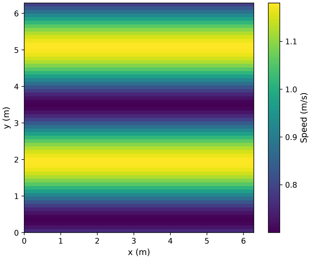
advected-shear-ibm 64x64: first z cell slice
