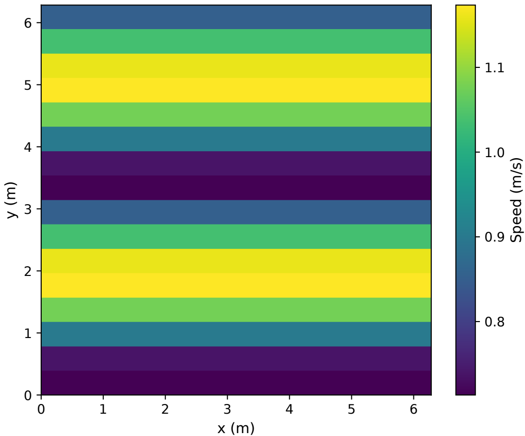
advected-shear 16x16x4: first z cell slice
