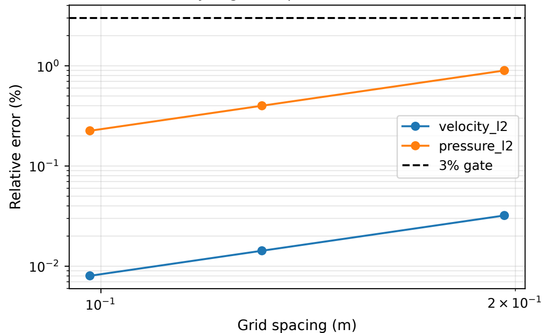
taylor-green: spatial refinement
