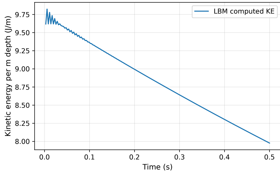
LBM energy diagnostic
