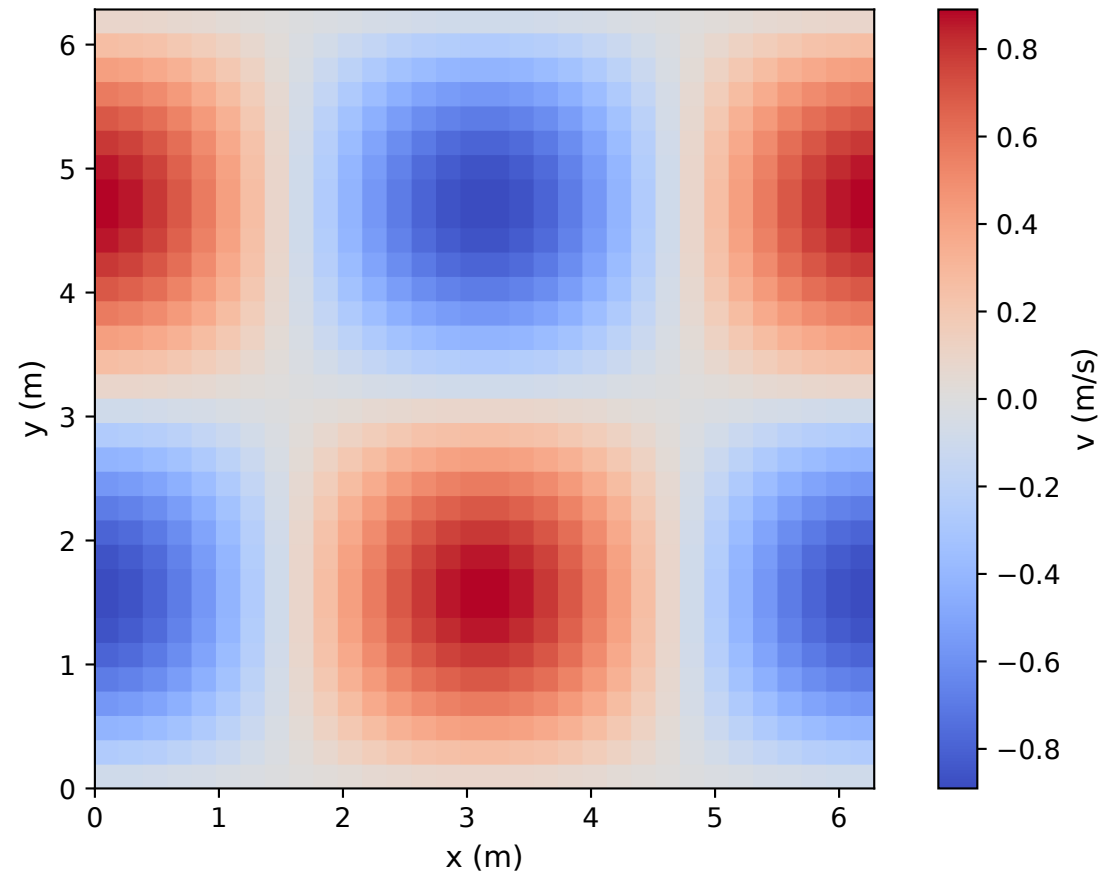
taylor-green-lbm: 32x32
