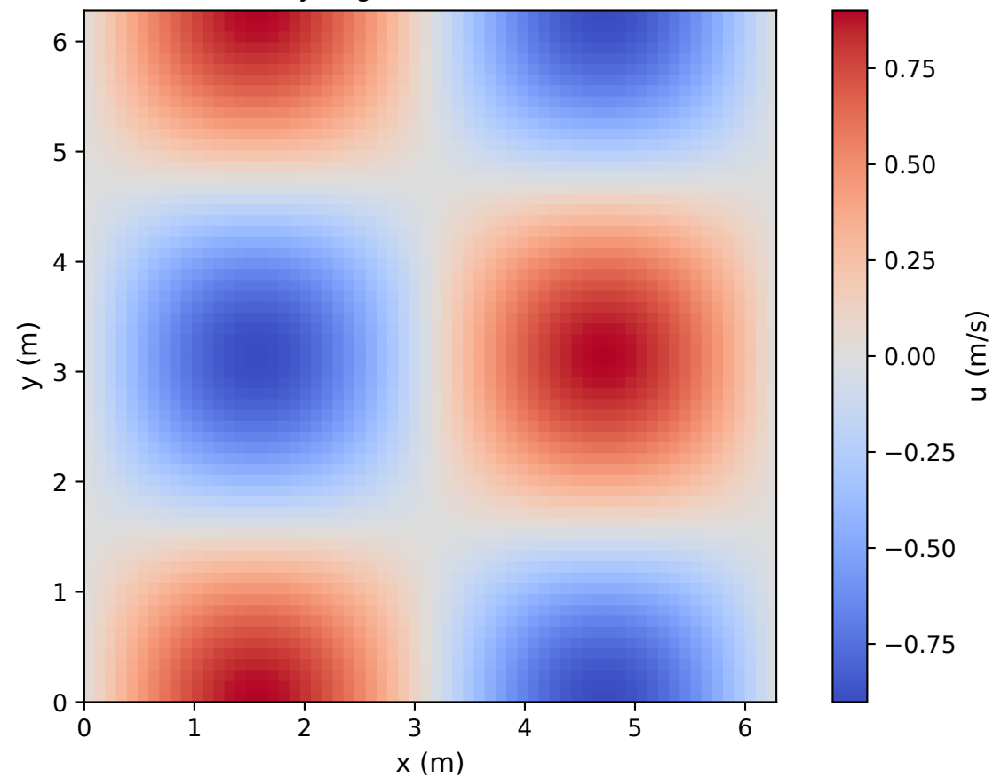
taylor-green-lbm: 64x64
