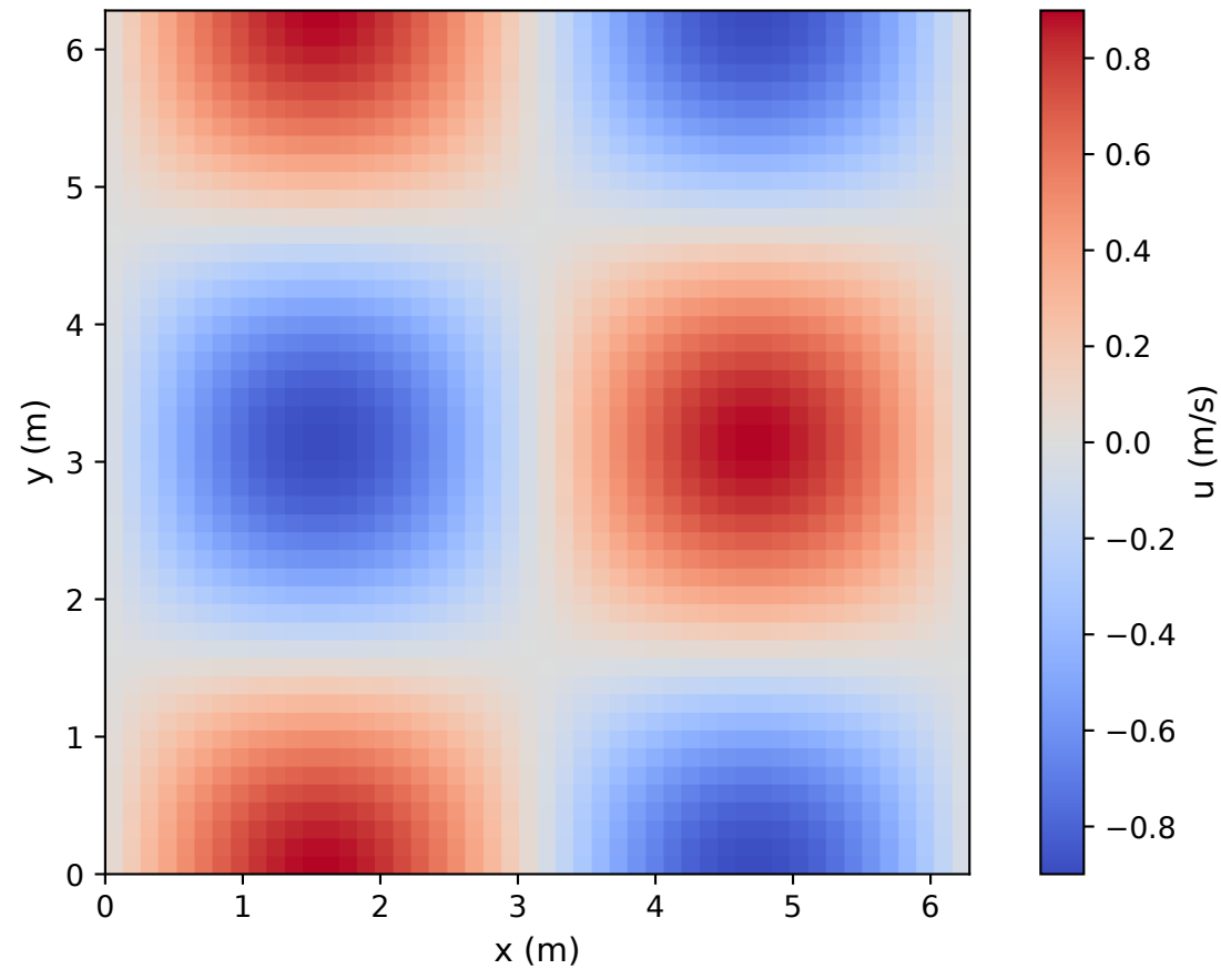
taylor-green: 48x48x4
