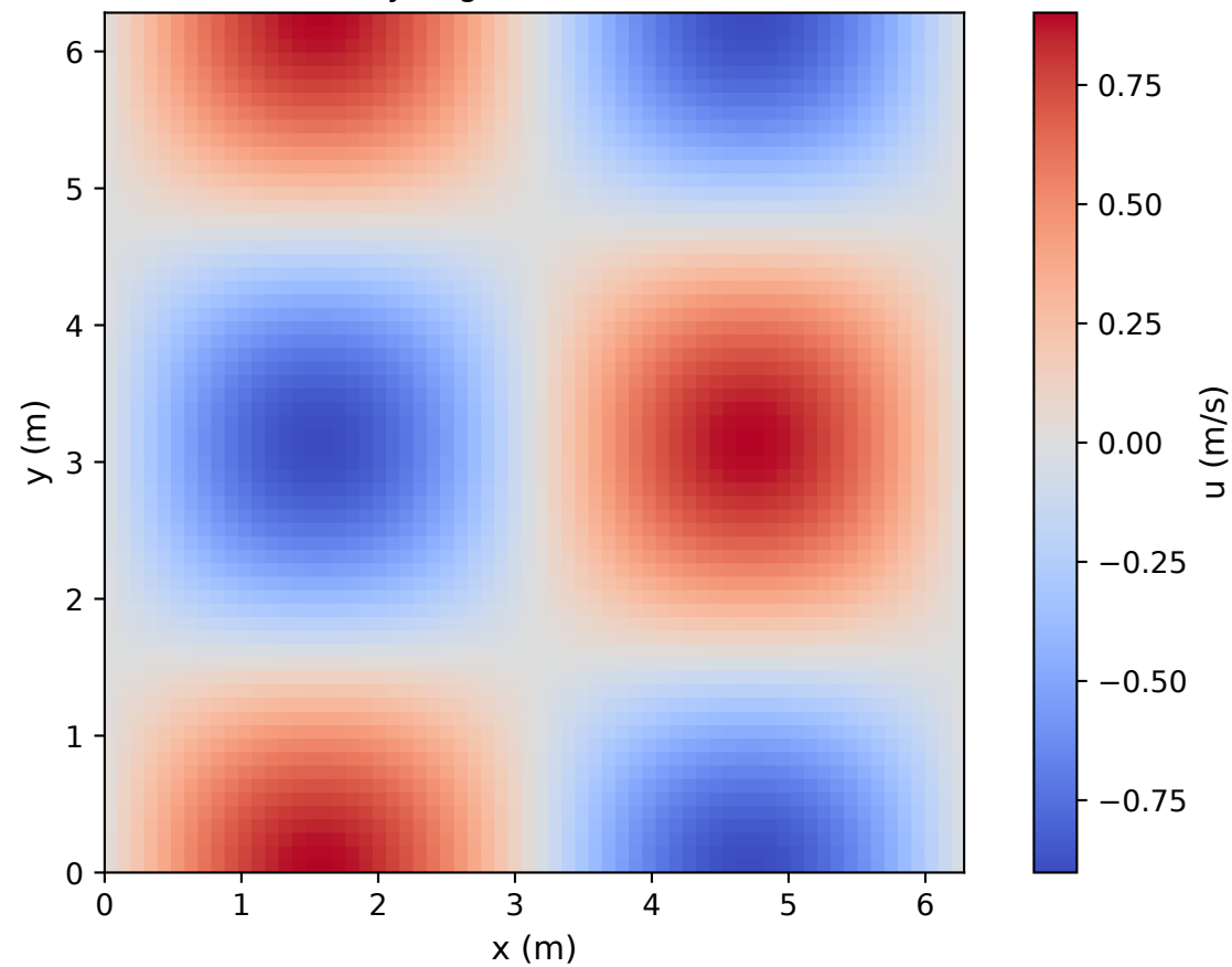
taylor-green: 64x64x4
