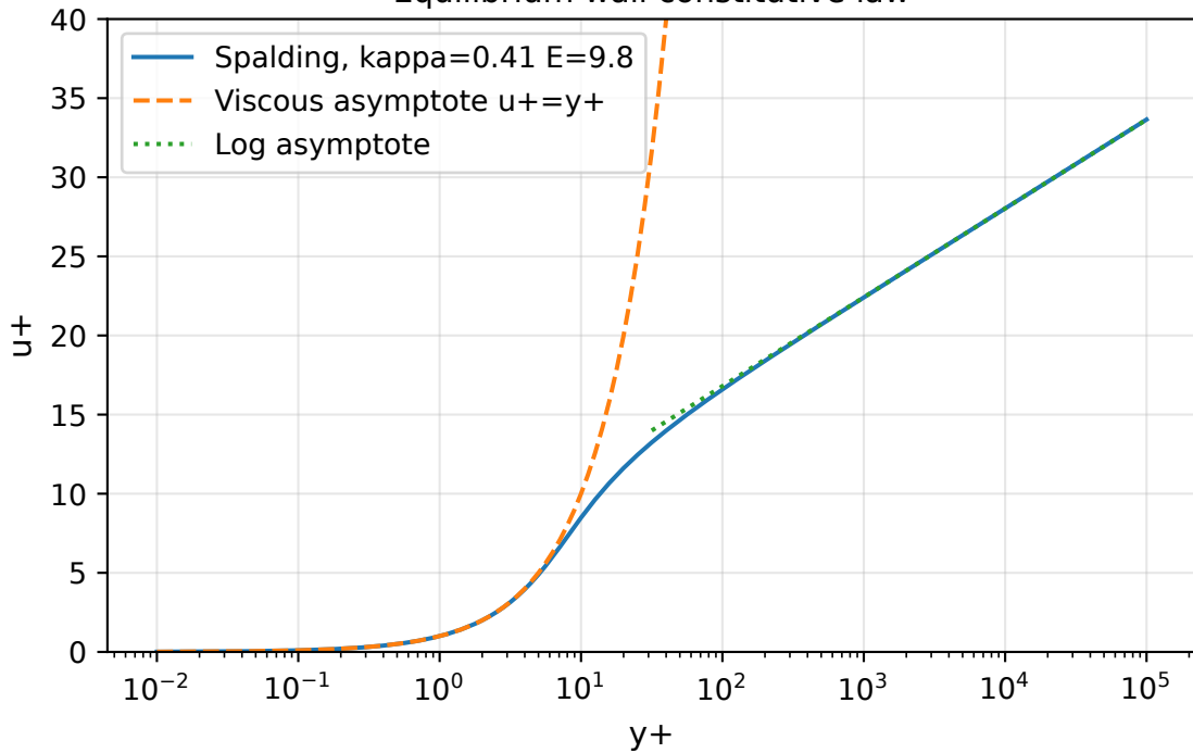
Equilibrium wall constitutive law
