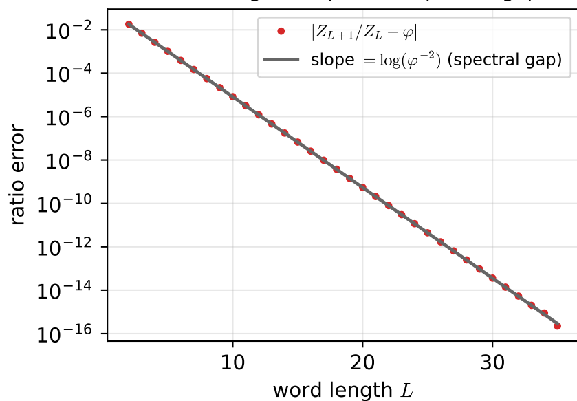
(b) convergence speed = spectral gap
