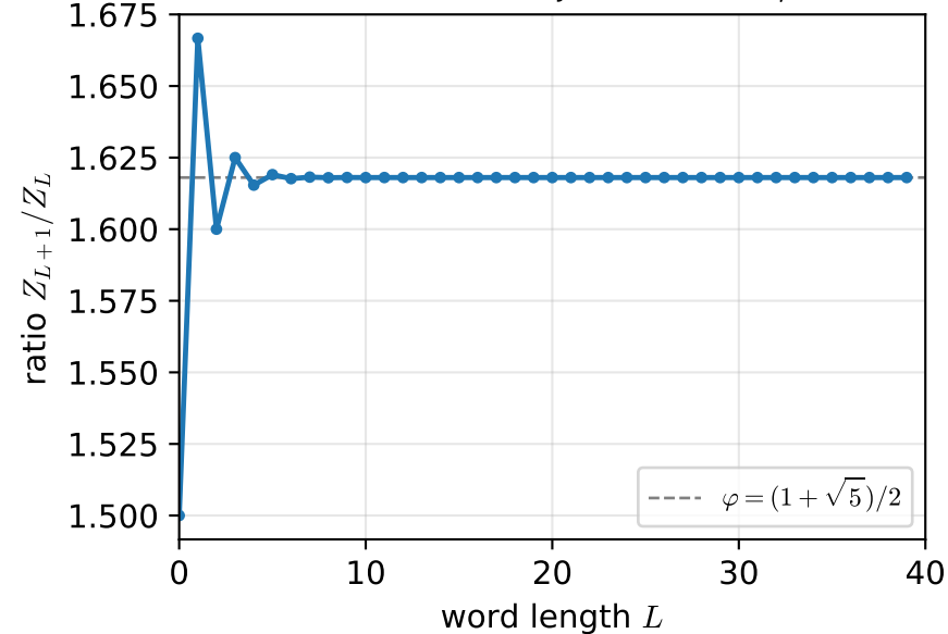
(a) ratio \rightarrow conjectured rate \varphi
