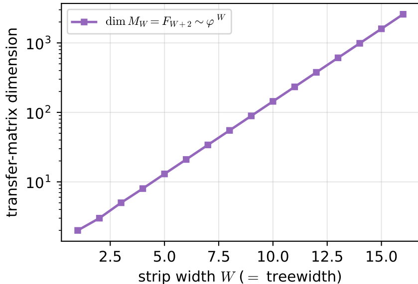
(b) cost = \Theta(q^{\text{tw}+1}L) grows with width
