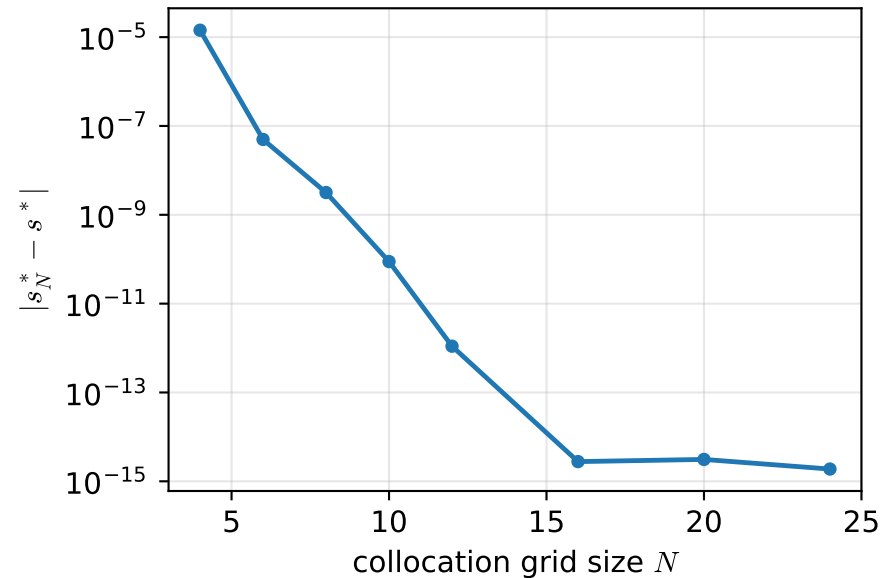
(a) operator route: spectral convergence to \dim_H E_2
