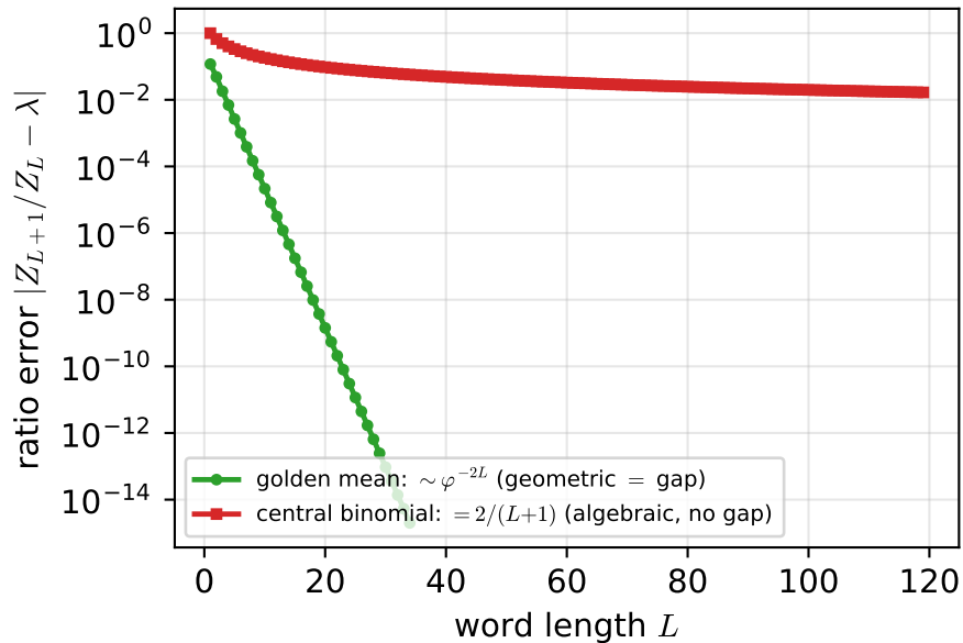
(b) ratio settles geometrically (gap) vs \sim 1/L (no gap)
