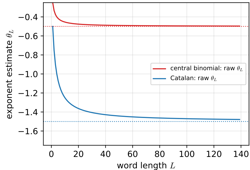
(a) raw ratio method \theta_L = L(r_L/\lambda - 1)
