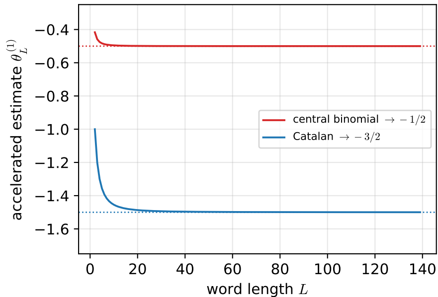
(b) one Richardson step pins the exponent
