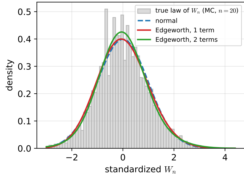
(a) Edgeworth captures the skew, n = 20
