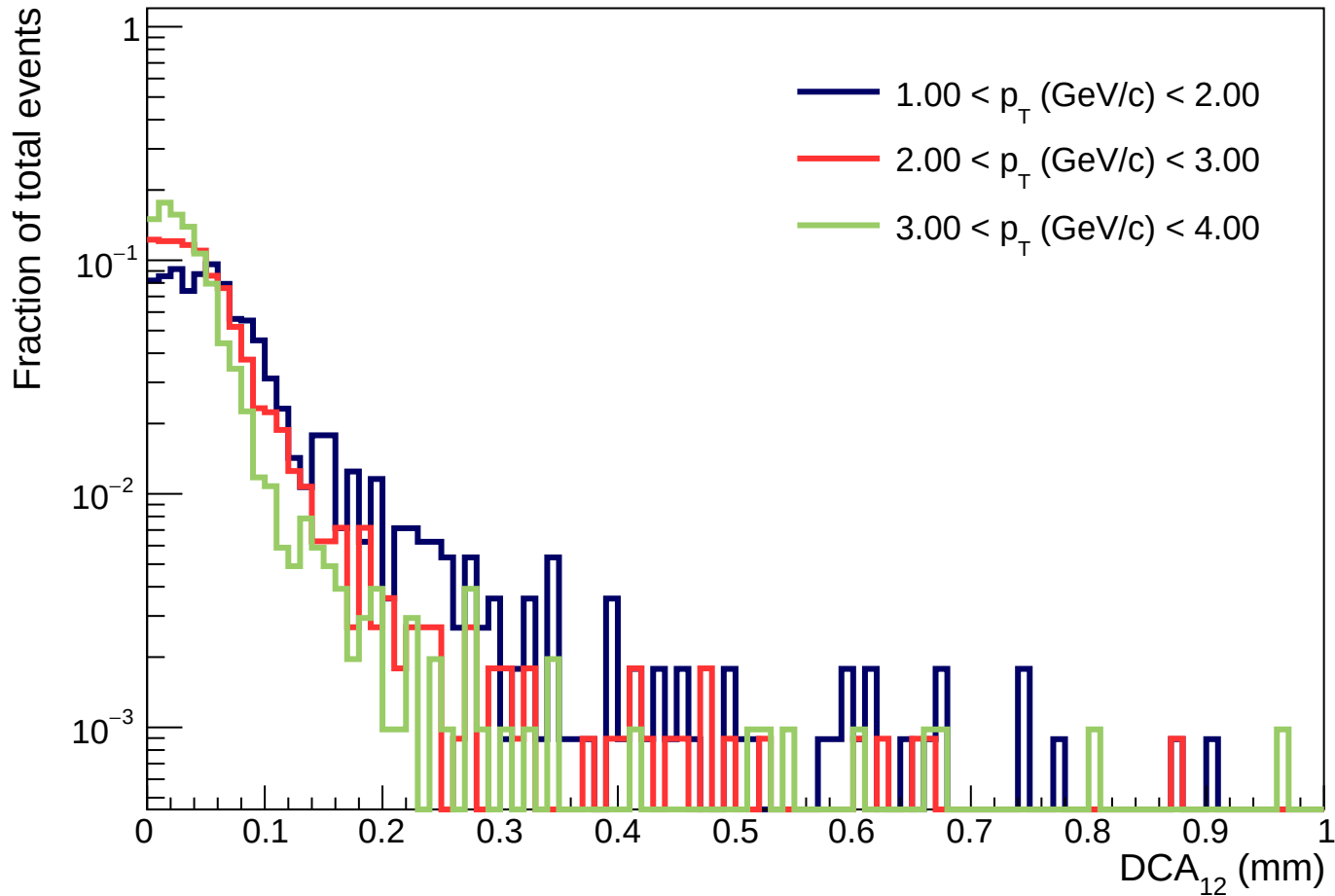
DCA 12 of \pi K pair for Q^2 > 100 signal ( -1 < y < 1 )
