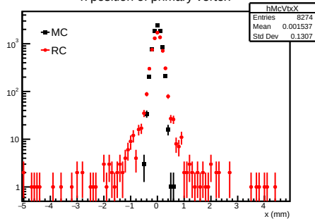
x position of primary vertex
