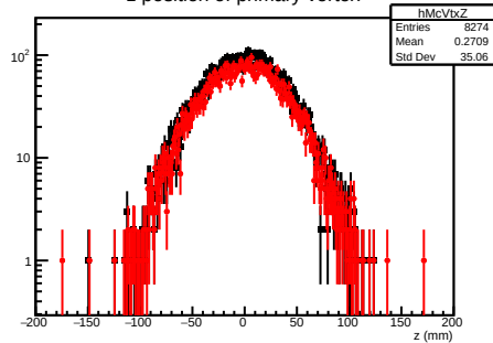
z position of primary vertex
