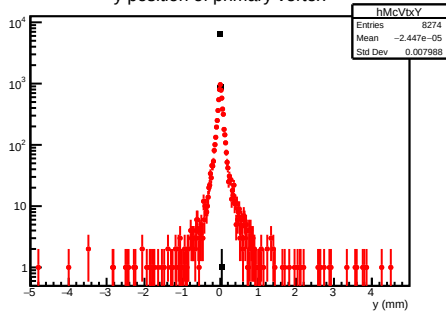
y position of primary vertex
