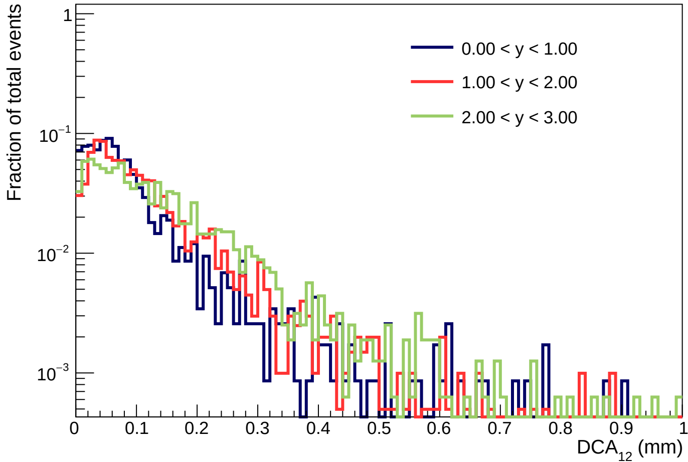
DCA 12 of \pi K pair for Q^2 > 100 signal ( 0 < p_T (GeV/c) < 2 )
