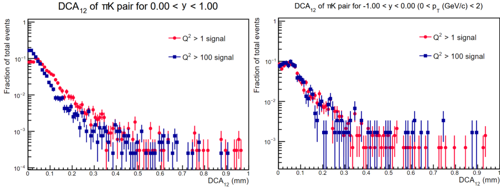
Figure 3.8: Comparison of DCA_{12} distributions between Q^2 > 1 \text{ GeV}^2 and Q^2 > 100 \text{ GeV}^2 ep collisions for reconstructed D^0 -mesons with any p_T (left) vs. with 0 < p_T < 2 \text{ GeV}/c , both at mid- y .
