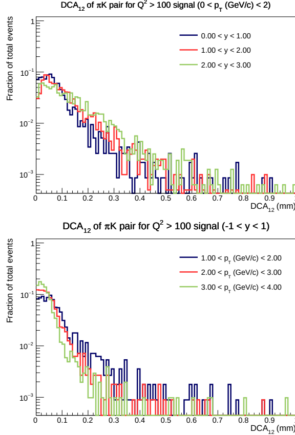
Figure 3.5: Examples of the y - and p_T -dependence of \text{DCA}_{12} of reconstructed D^0 -mesons in simulated Q^2 > 100 \text{ GeV}^2 ep collisions. The top plot compares distributions in various y ranges for 0 < p_T < 2 \text{ GeV}/c , and the bottom plot compares distributions in various p_T ranges for -1 < y < 1 .
