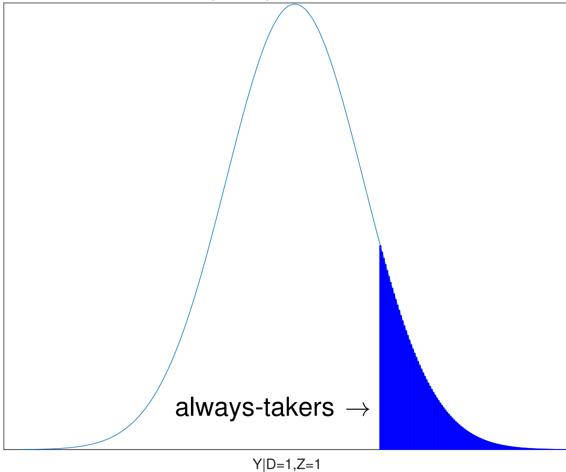
Probability density function for Y|D=1, Z=1
