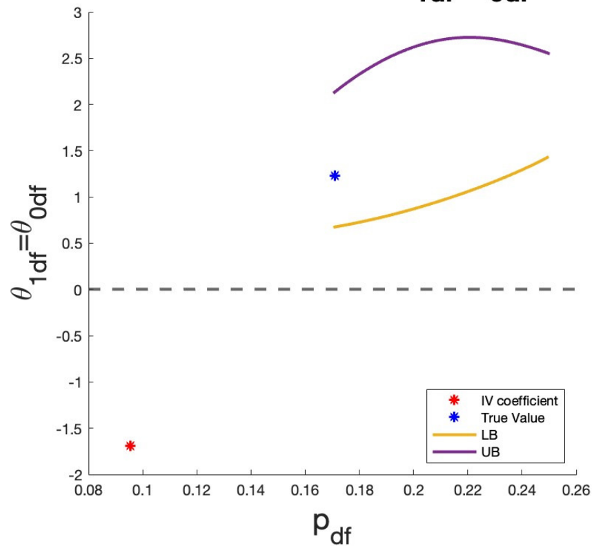
Identified set for \theta_{1df} = \theta_{0df}
