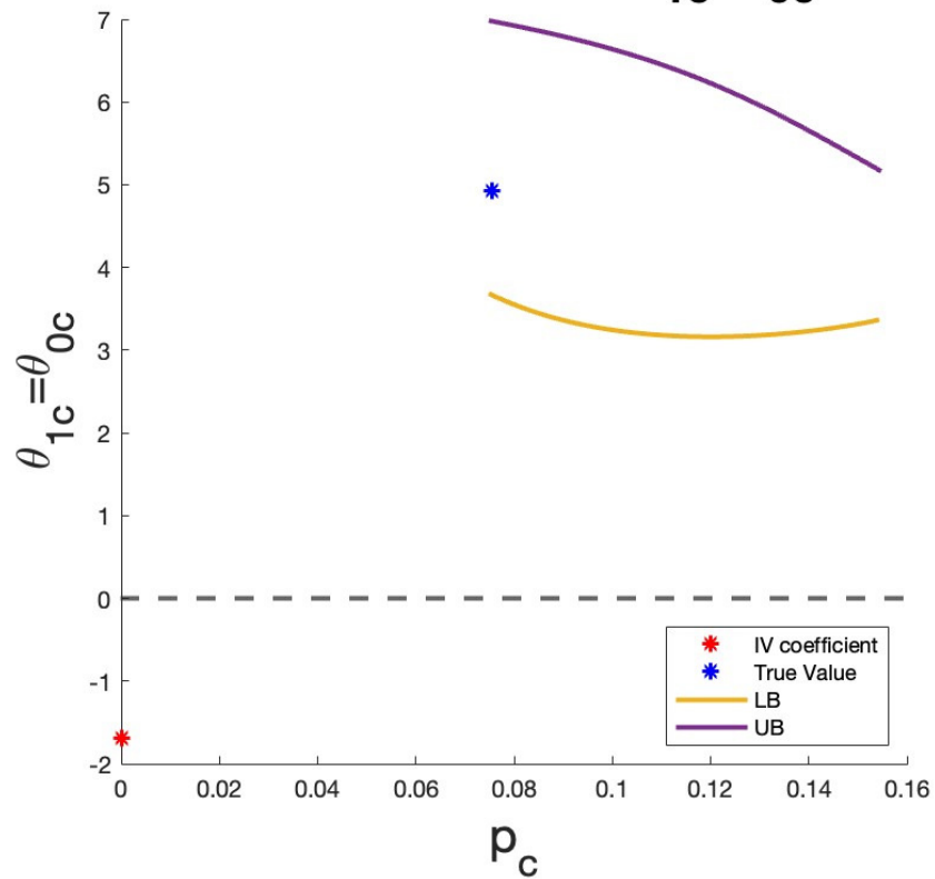
Identified set for \theta_{1c} = \theta_{0c}
