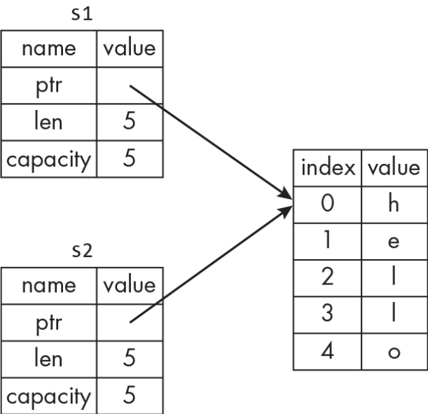
Figure 4-2: The representation in memory of the variable s2 that has a copy of the pointer, length, and capacity of s1
