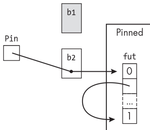
Figure 17-7: Moving a Box that points to a self-referential future type
