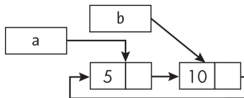
Figure 15-4: A reference cycle of lists a and b pointing to each other
