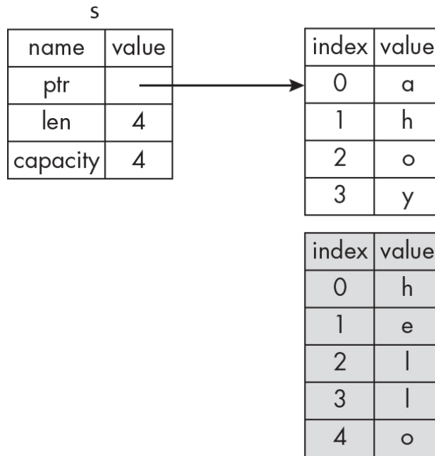
Figure 4-5: The representation in memory after the initial value has been replaced in its entirety
