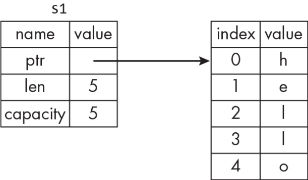
Figure 4-1: The representation in memory of a String holding the value "hello" bound to s1
