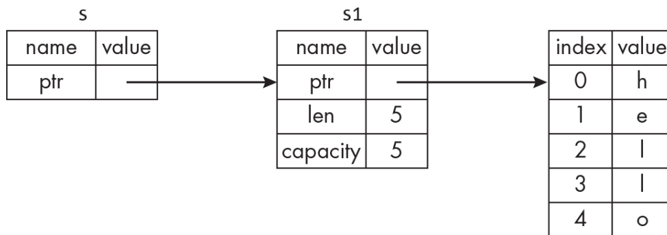
Figure 4-6: A diagram of &String s pointing at String s1
