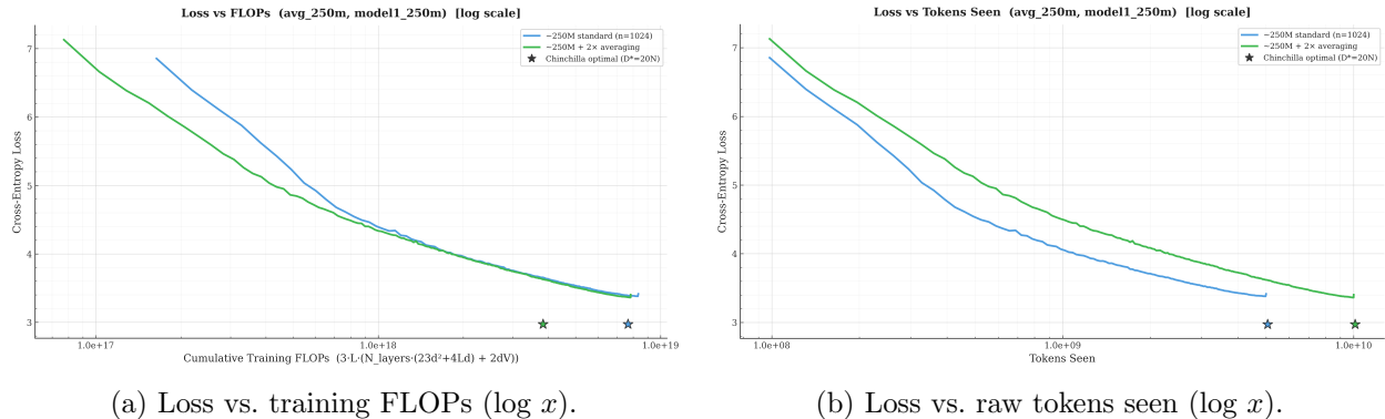
Figure 3: 250M comparison on native eval losses, both arms at their full budgets (5B and 10B raw tokens). The picture matches the smaller scales: the k=2 curve sits below the baseline at equal FLOPs throughout, and slightly above it on the raw-token axis. The gap at the end is visibly narrower here than at 125M, which is what the shrinking efficiency multiplier looks like.
