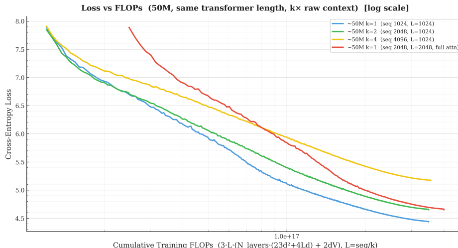
Figure 5: Context experiment at 50M: native eval loss vs. training FLOPs (log x ). Curves with different k score different sets of positions and are overlaid only for orientation; the valid comparisons are within one method (see text). The two arms with 2048 tokens of raw context (green: k=2 averaging; red: full attention) end at almost the same native loss at very different cost, and 4\times context (yellow) is worse still. Early-training loss spikes are clipped at 8.0 for readability.
