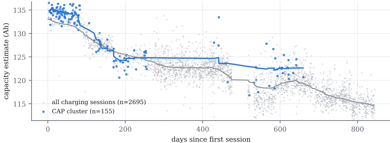
Vehicle 3: scatter about the ageing trend 1.68% \rightarrow 1.32%
