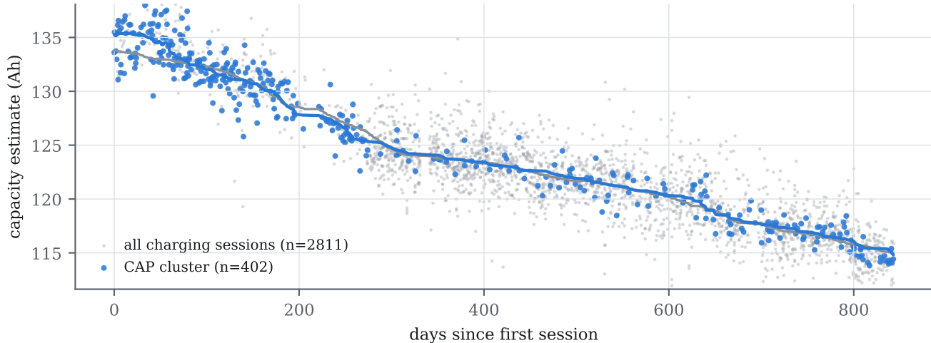
Vehicle 1: scatter about the ageing trend 1.45% \rightarrow 1.03%
