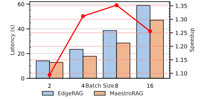
Figure 5: Latency comparison of EdgeRAG and MaestroRAG on a Jetson AGX Orin with 1 M database.
