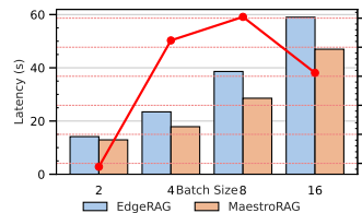
Figure 5: Latency comparison of EdgeRAG and MaestroRAG on a Jetson AGX Orin with 1M database.
