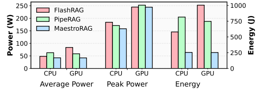
Figure 6: Power and energy comparison of the three schemes measured on Intel i9-14900K platform with RTX 4090 GPU with \text{BS}=2 , \text{DB}=4\text{M} and \text{top-k}=5 .
