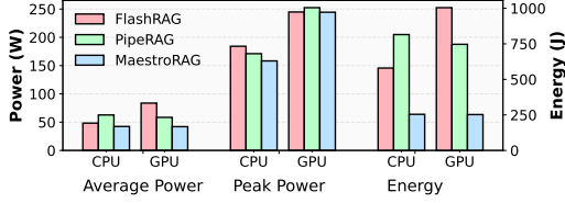
Figure 6: Power and energy comparison of the three schemes measured on Intel i9-14900K platform with RTX 4090 GPU with BS=2, DB=4 M and top-k=5.
