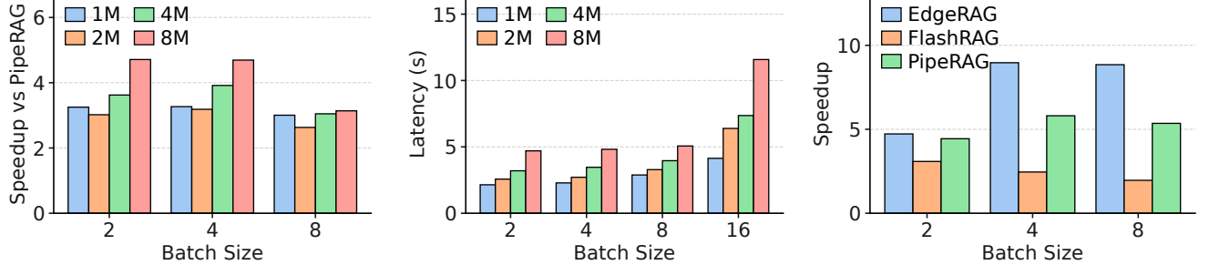
(d) Speedup: MaestroRAG vs PipeRAG [16]. (e) E2E latency of MaestroRAG in RTX 4080 (f) Speedup: MaestroRAG vs other baselines.
