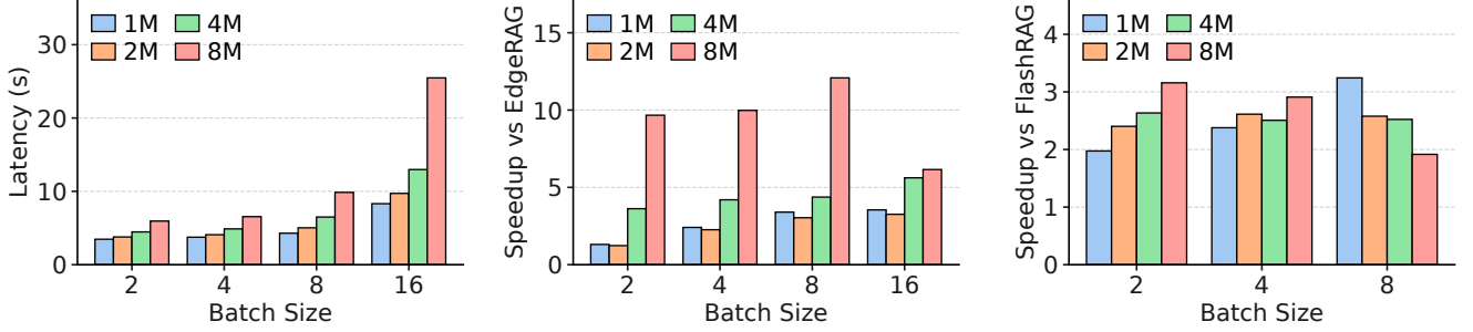
(a) E2E latency of MaestroRAG in RTX4090. (b) Speedup: MaestroRAG vs EdgeRAG [37]. (c) Speedup: MaestroRAG vs FlashRAG [19].
