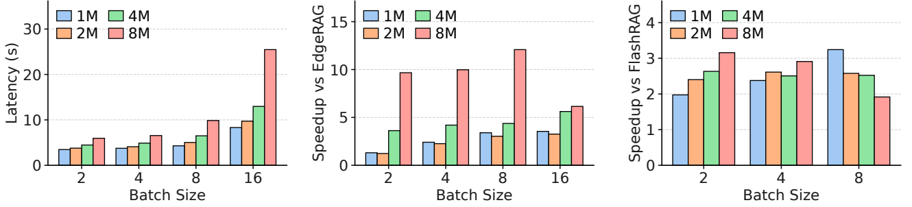
(a) E2E latency of MaestroRAG in RTX4090. (b) Speedup: MaestroRAG vs EdgeRAG [34]. (c) Speedup: MaestroRAG vs FlashRAG [18].
