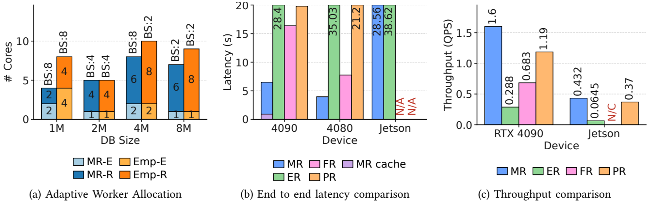
Figure 6: (a) Core allocation chosen by the adaptive worker allocator against the allocation found by exhaustive search, for four database sizes; bar height is the total core count and the annotation gives the batch size. (b) End-to-end latency across the three platforms at the allocations in (a); the lower segment of the MaestroRAG bar on the RTX 4090 is the cached latency and the upper segment is the remainder of the uncached total. (c) Throughput across the same configurations. Bars marked N/A are configurations the baseline does not support. [FLAG: This caption does not state the operating point for panels (b) and (c). $5.5 gives BS=8 with 4 M, 4 M and 1 M databases, and $5.6 gives DB=4 M, BS=8. Add them here if the caption should stand alone.]
