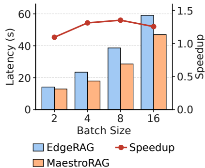
Figure 5: Latency comparison of EdgeRAG and MaestroRAG on a Jetson AGX Orin with 1 M database.
