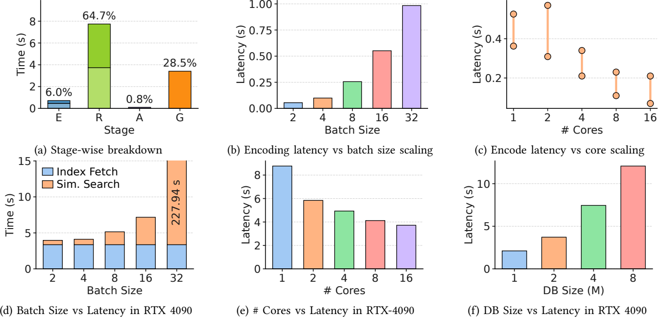
Figure 2: Characterizations: (a) Stage-wise breakdown of RAG pipeline. Lighter shades represent start-up cost and darker execution time. Characterization for encode stage (b–c): (b) Encode stage latency for different batch sizes on 8 cores. (c) Encode latency at batch size 16 as we vary the number of CPU cores. Characterization for retrieval stage (d–f): (d) Retrieval stage breakdown on 4 cores with different batch sizes ( Index Fetch vs. Similarity Search ). (e) Retrieval latency as the number of CPU cores increases (DB size = 2 M, batch size = 8). (f) Retrieval latency vs. database size (batch size = 8).
