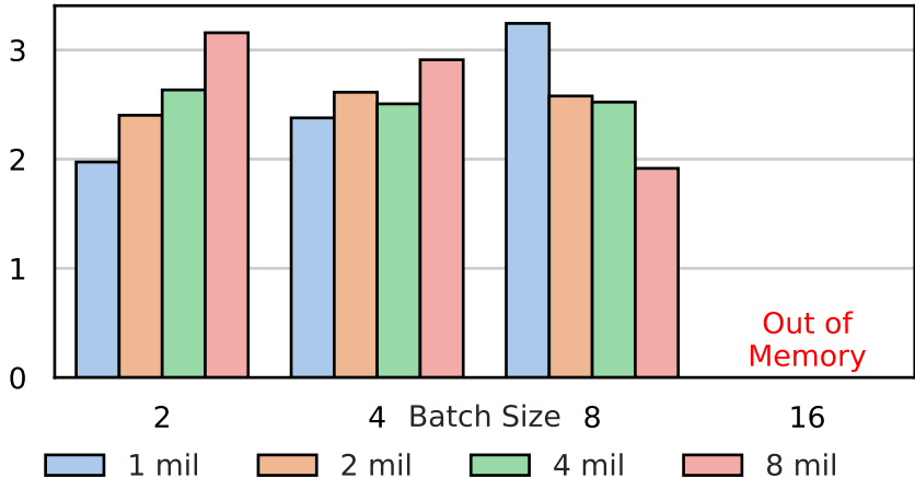
Speedup vs FlashRAG
