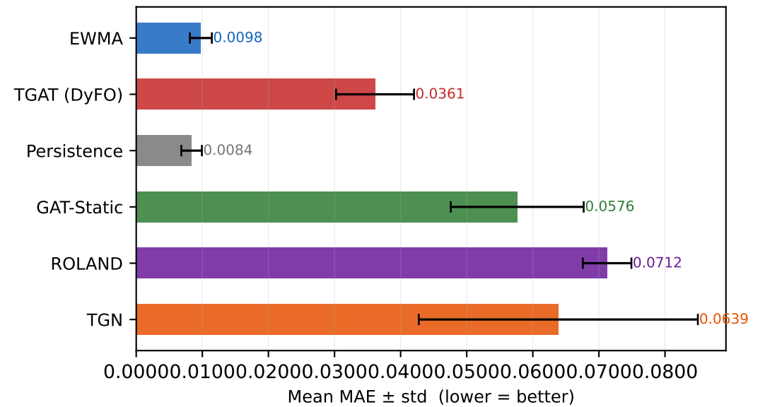
Aggregate MAE
