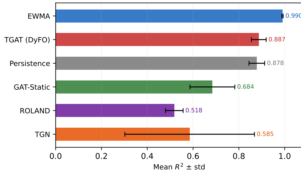
Aggregate R^2
