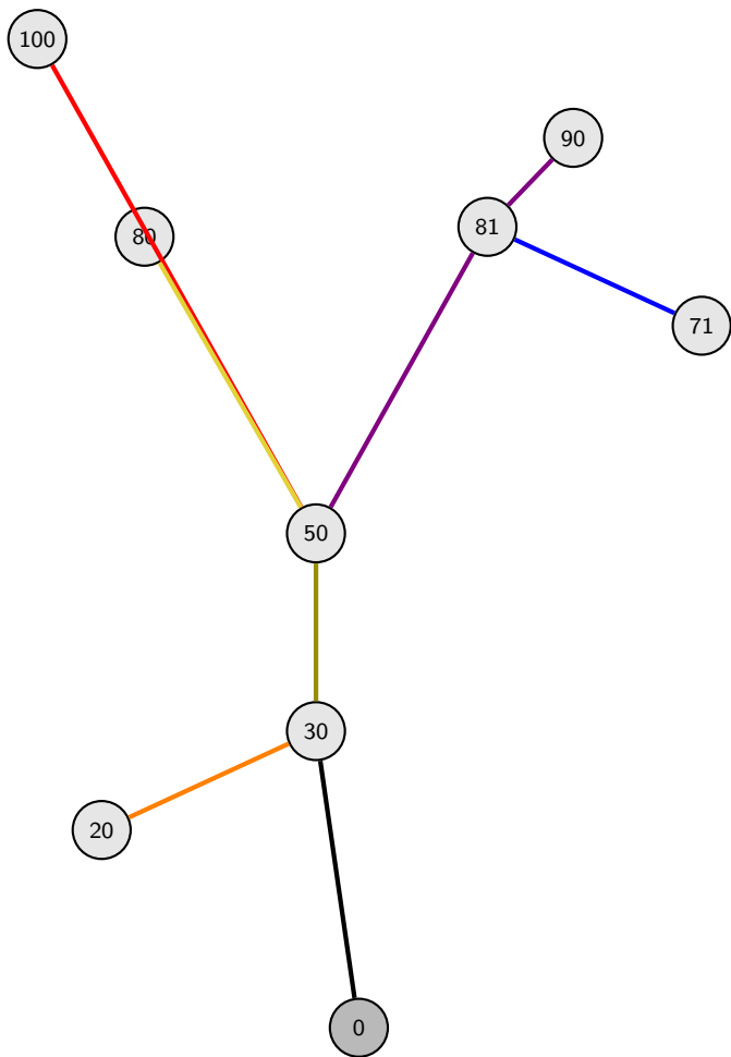
Full Tree (Contour / Augmented Tree)
