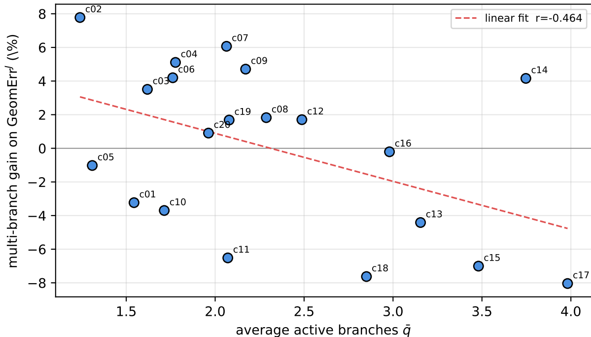
multi-branch weighting gain vs. average active branches (target compression=50%, \alpha=0.5 )
