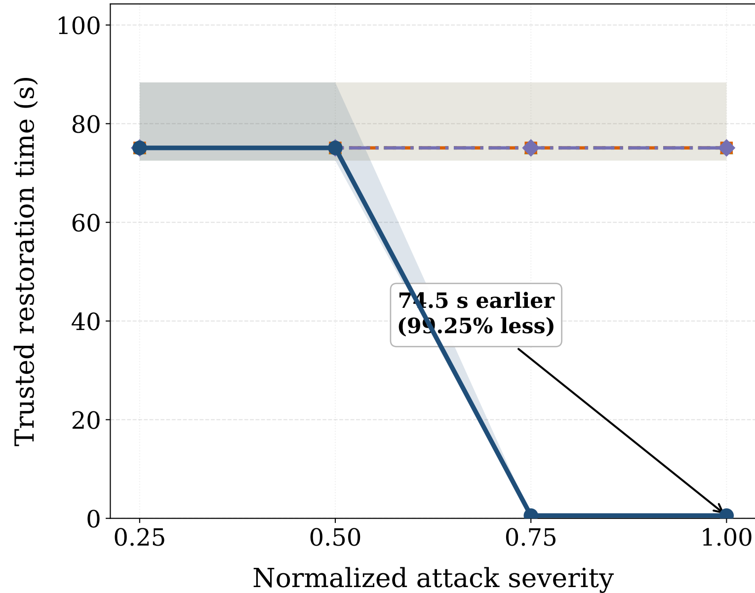
(b) HVAC Attacks (Additive Bias + Drift)
