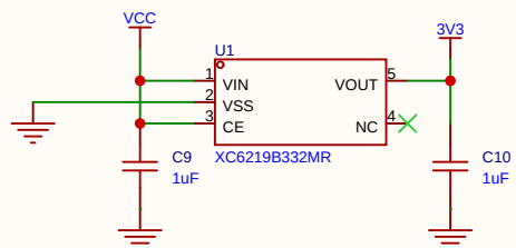
LDO线性降压
