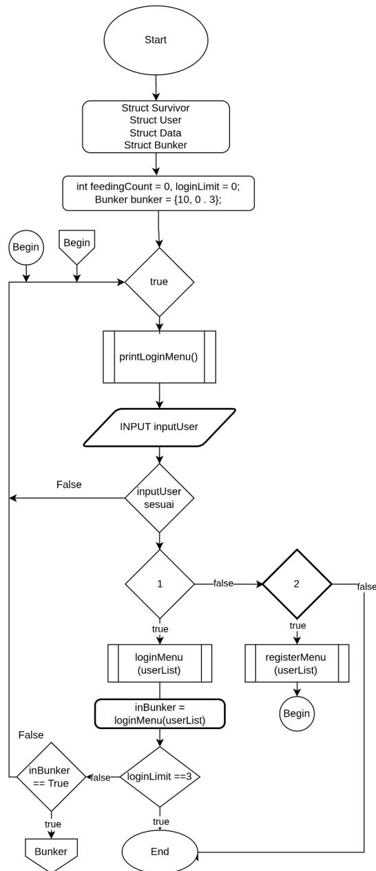
Gambar 1.1. Flowchart Menu Awal
