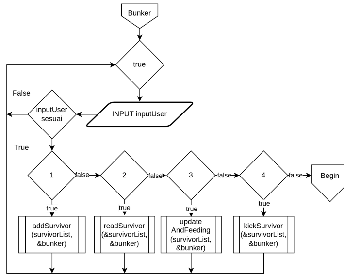
Gambar 1.3. Flowchart Menu Bunker
