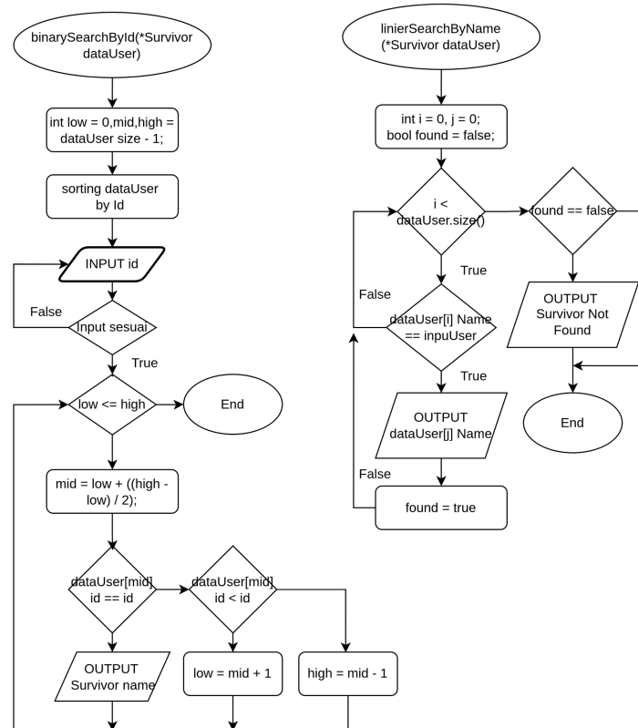
Gambar 1.8. Flowchart Prosedur Searching
