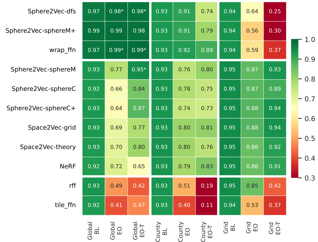
Pattern Recovery (Pearson r)
